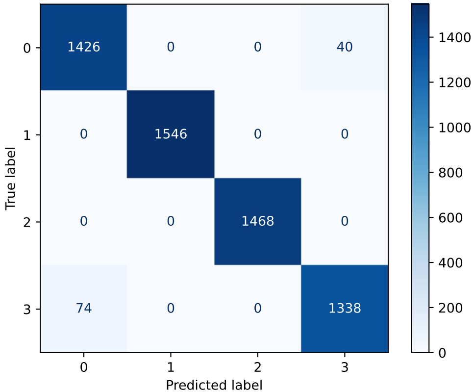
Fold 1 - Confusion Matrix
